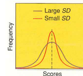
Figure 2.9 Standard Deviation
